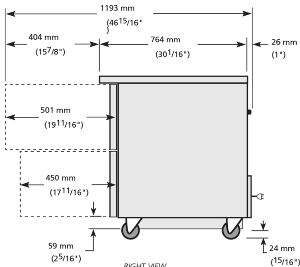
RIGHT VIEW
