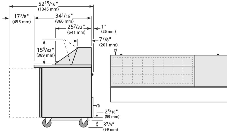
RIGHT VIEW
