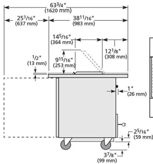
RIGHT VIEW
