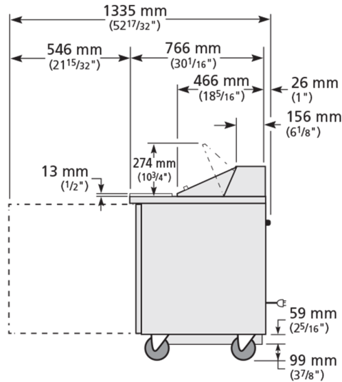
RIGHT VIEW
