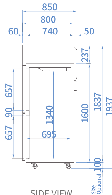
SIDE VIEW (Half Door)
