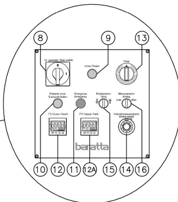
CONTROL PANEL
