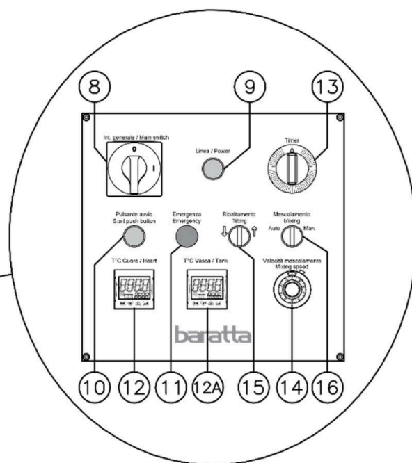
CONTROL PANEL
