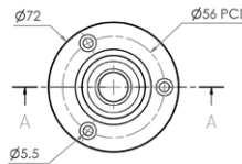
Mounting Body
